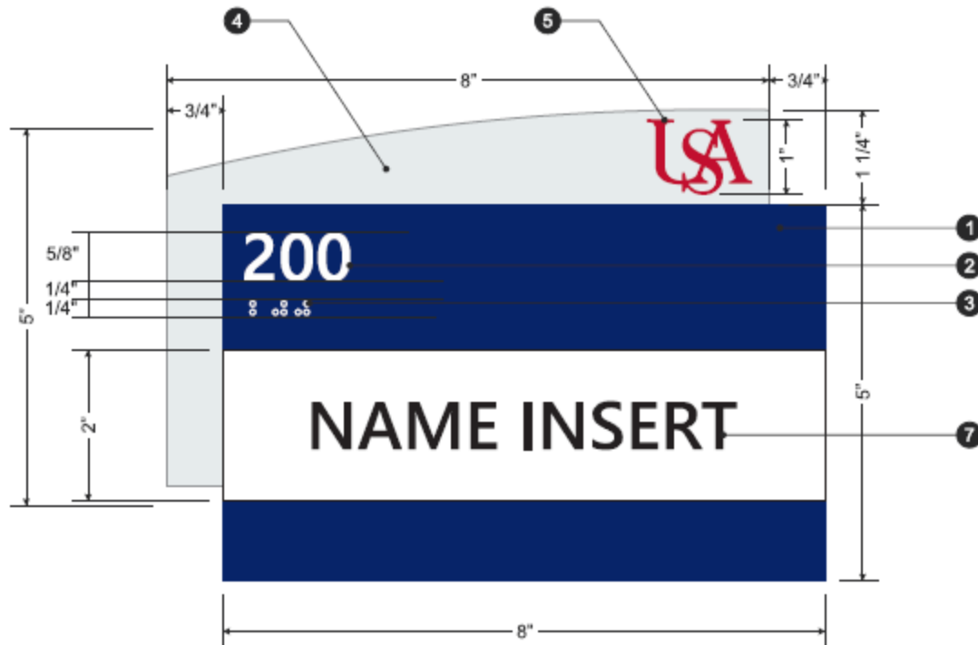
Front View Scale: 1/2 of Actual Size
