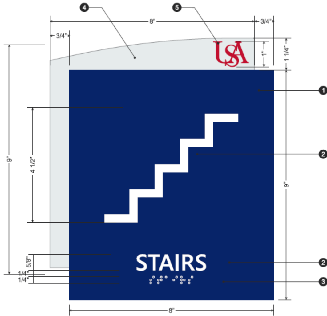
Front View Scale: 1/2 of Actual Size
