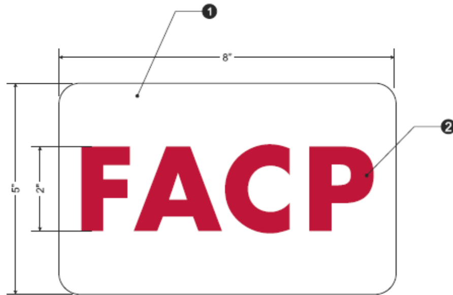
Front View Scale: 1/2 of Actual Size
